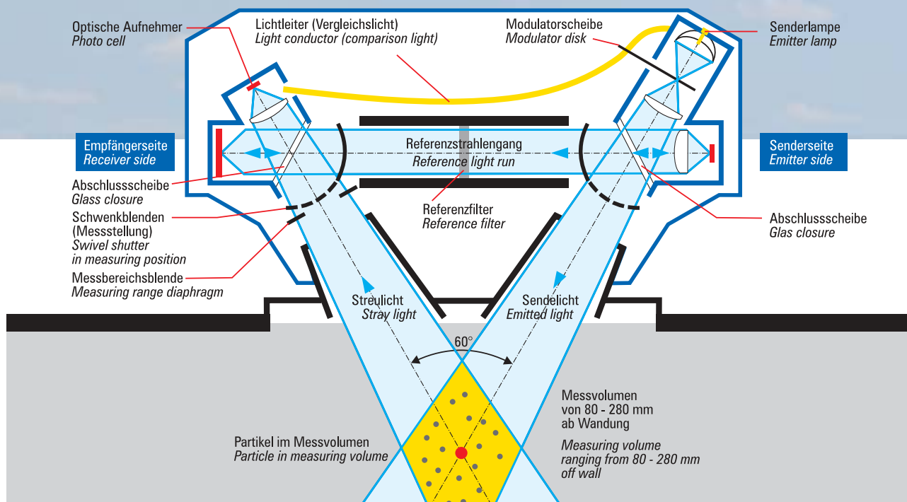
Messprinzip D-R 300/300-40 D-R 300/300-40 Measuring Principle
